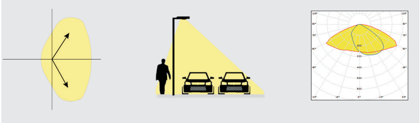
TYPE 3
